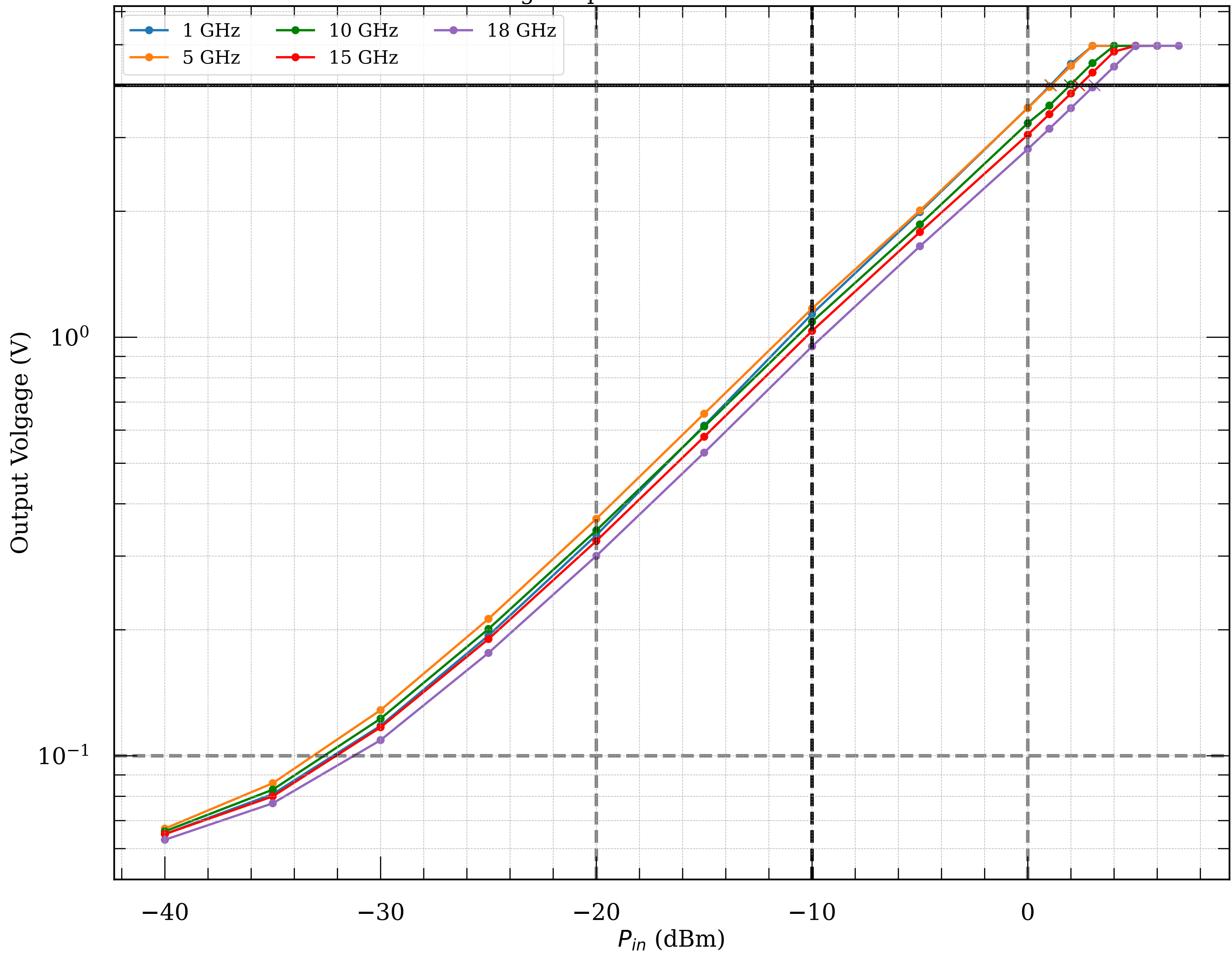
Measured voltage-to-power curve of detector module031
